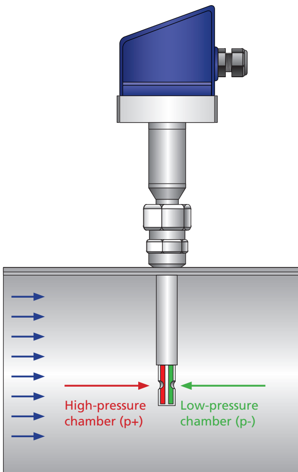
Functional principle of deltaflowC probe
